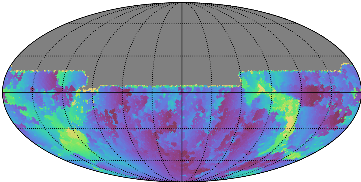
mw_roll_bulge_v3.3_10yrs All sky u band: Min solarElong
