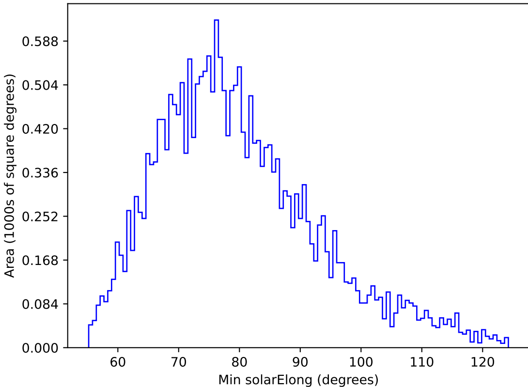
mw_roll_bulge_v3.3_10yrs All sky u band: Min solarElong
