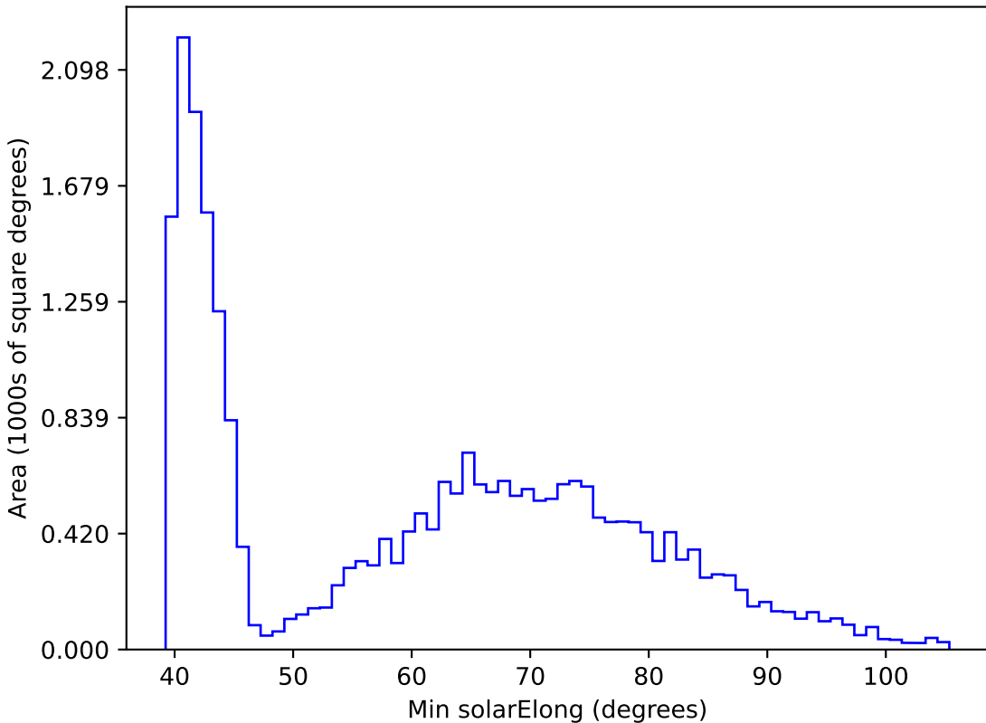
mw_roll_bulge_v3.3_10yrs All sky r band: Min solarElong
