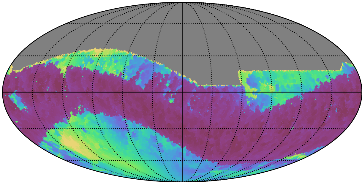
mw_roll_bulge_v3.3_10yrs All sky i band: Min solarElong
