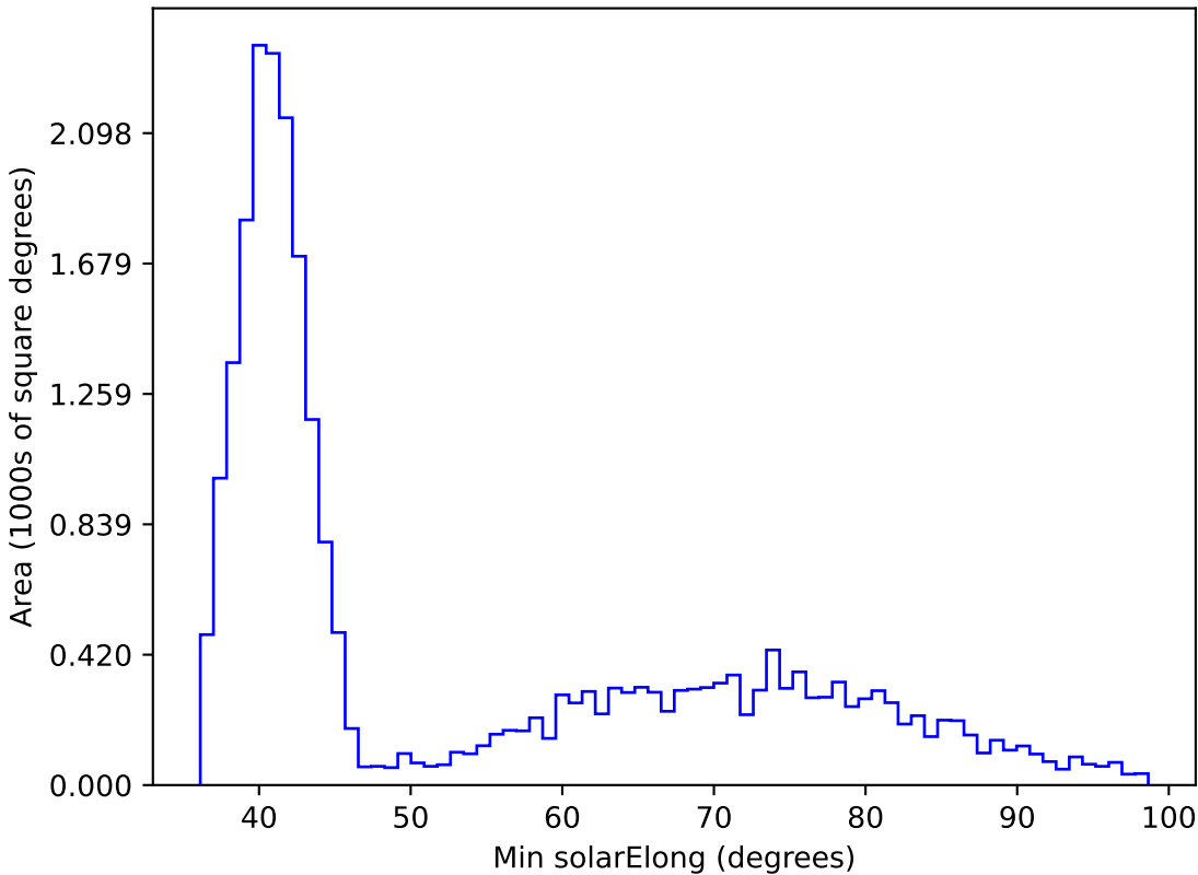
mw_roll_bulge_v3.3_10yrs All sky i band: Min solarElong
