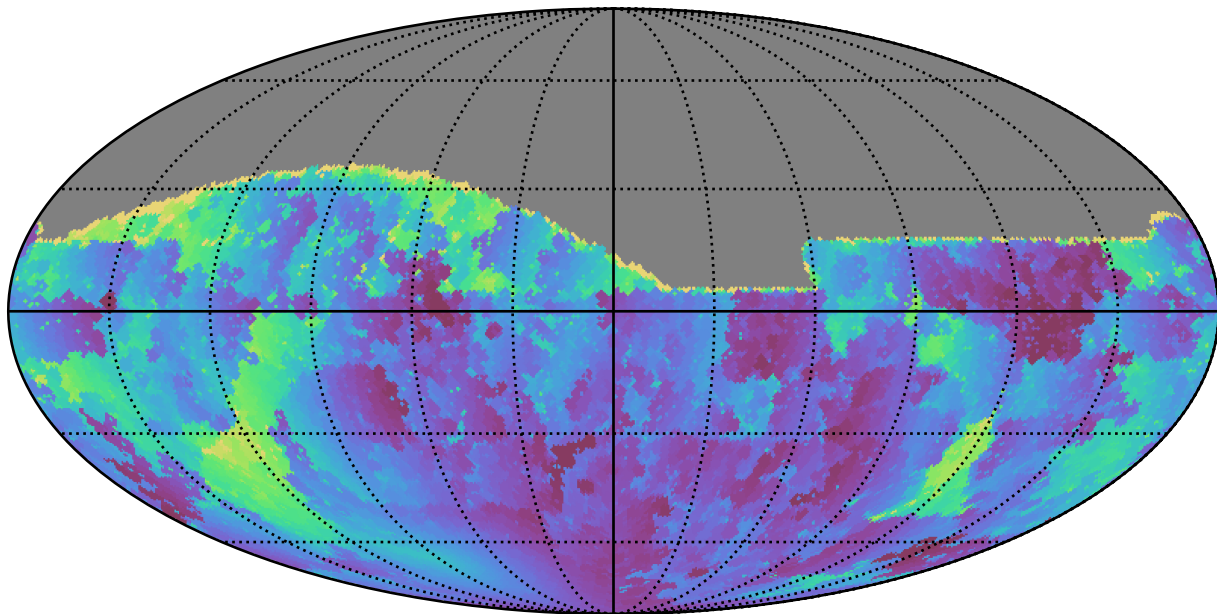
mw_roll_bulge_v3.3_10yrs All sky g band: Min solarElong
