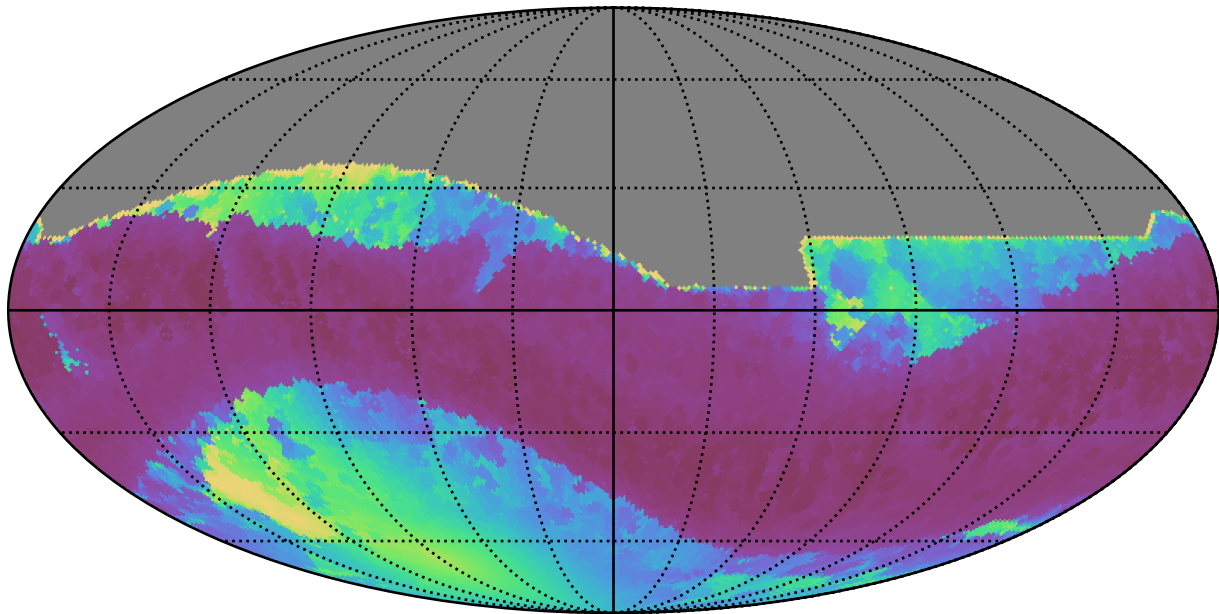
mw_roll_bulge_v3.3_10yrs All sky all bands: Min solarElong
