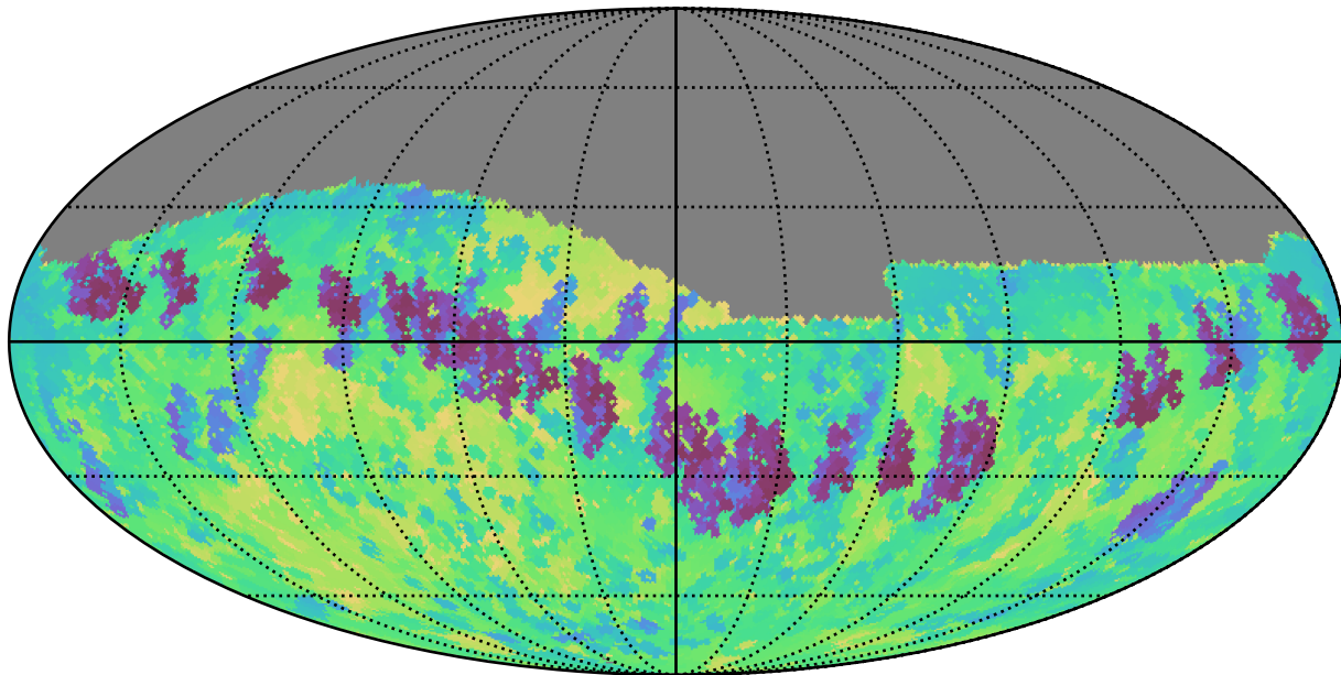
mw_roll_bulge_v3.3_10yrs Yr1 z band: Min skyBrightness
