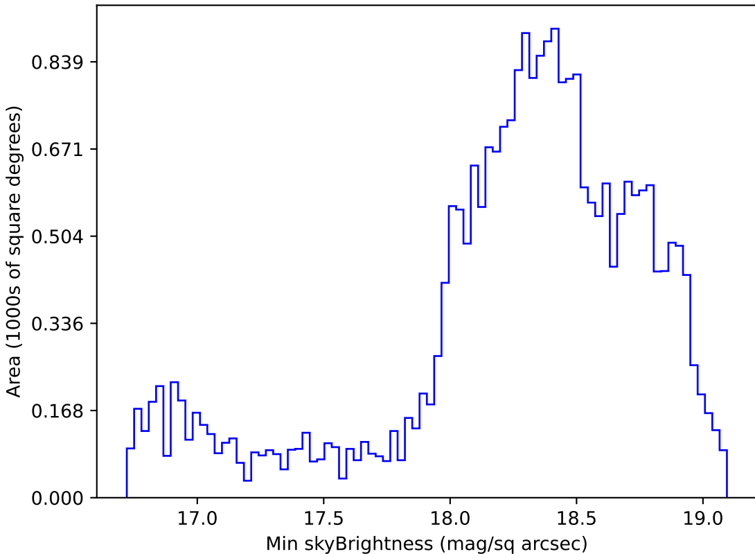
mw_roll_bulge_v3.3_10yrs Yr 1 z band: Min skyBrightness
