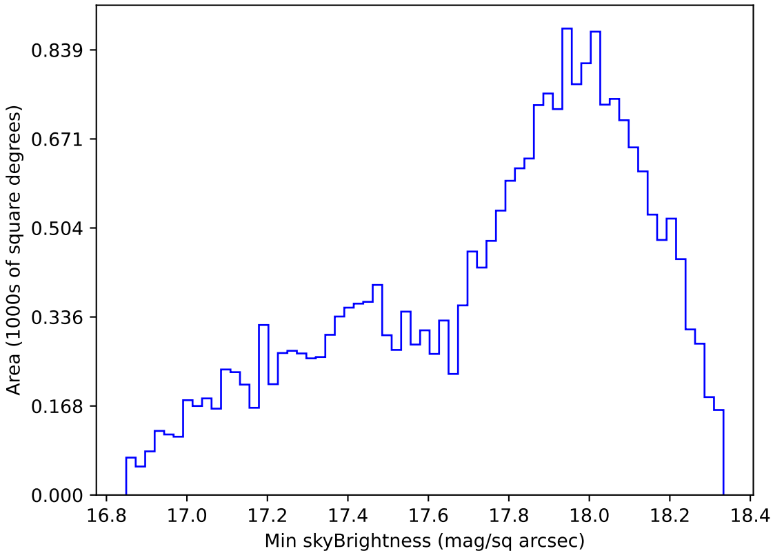
mw_roll_bulge_v3.3_10yrs Yr 1 y band: Min skyBrightness
