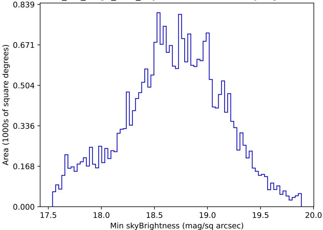
mw_roll_bulge_v3.3_10yrs Yr 1 i band: Min skyBrightness
