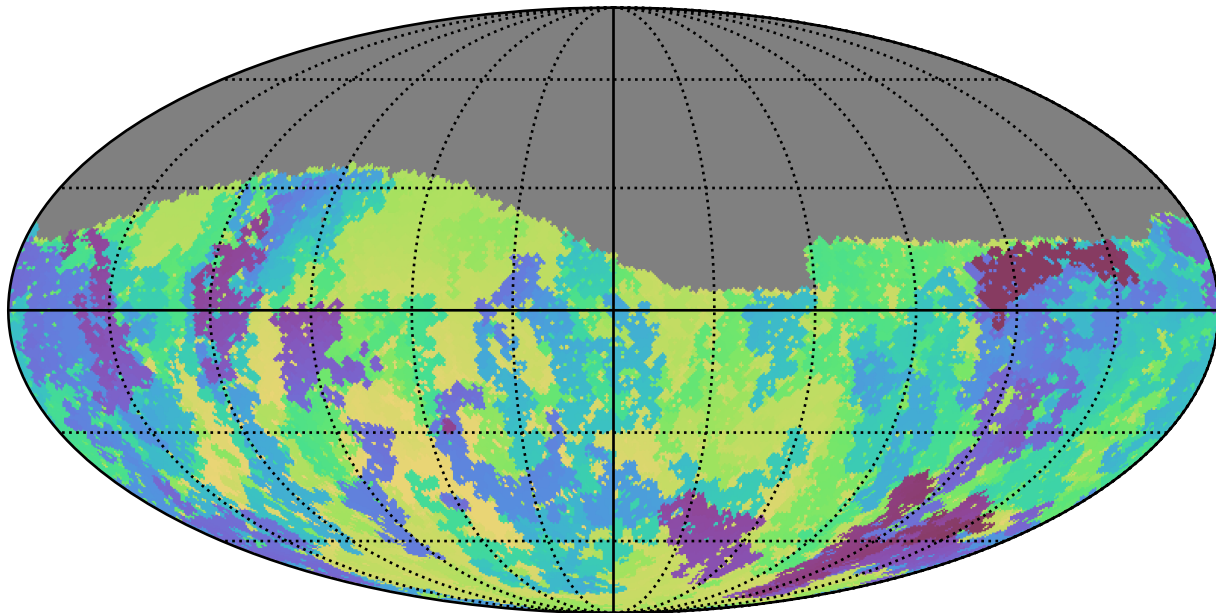
mw_roll_bulge_v3.3_10yrs Yr 1 g band: Min skyBrightness
