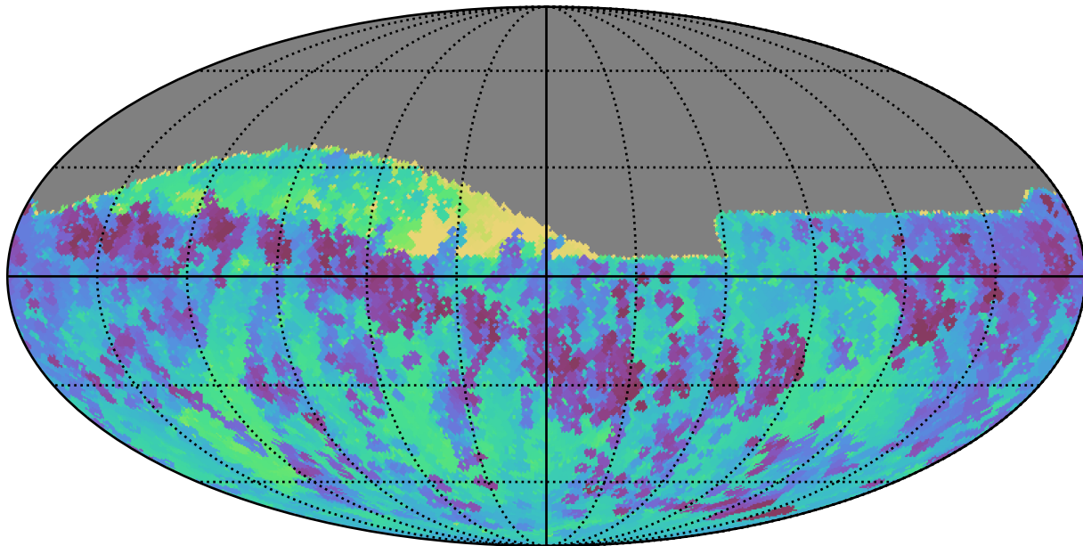
mw_roll_bulge_v3.3_10yrs Yr 1 all bands: Min skyBrightness
