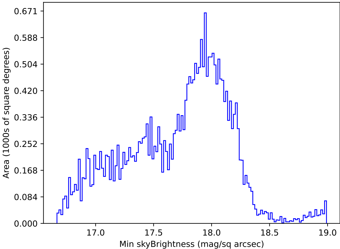
mw_roll_bulge_v3.3_10yrs Yr 1 all bands: Min skyBrightness
