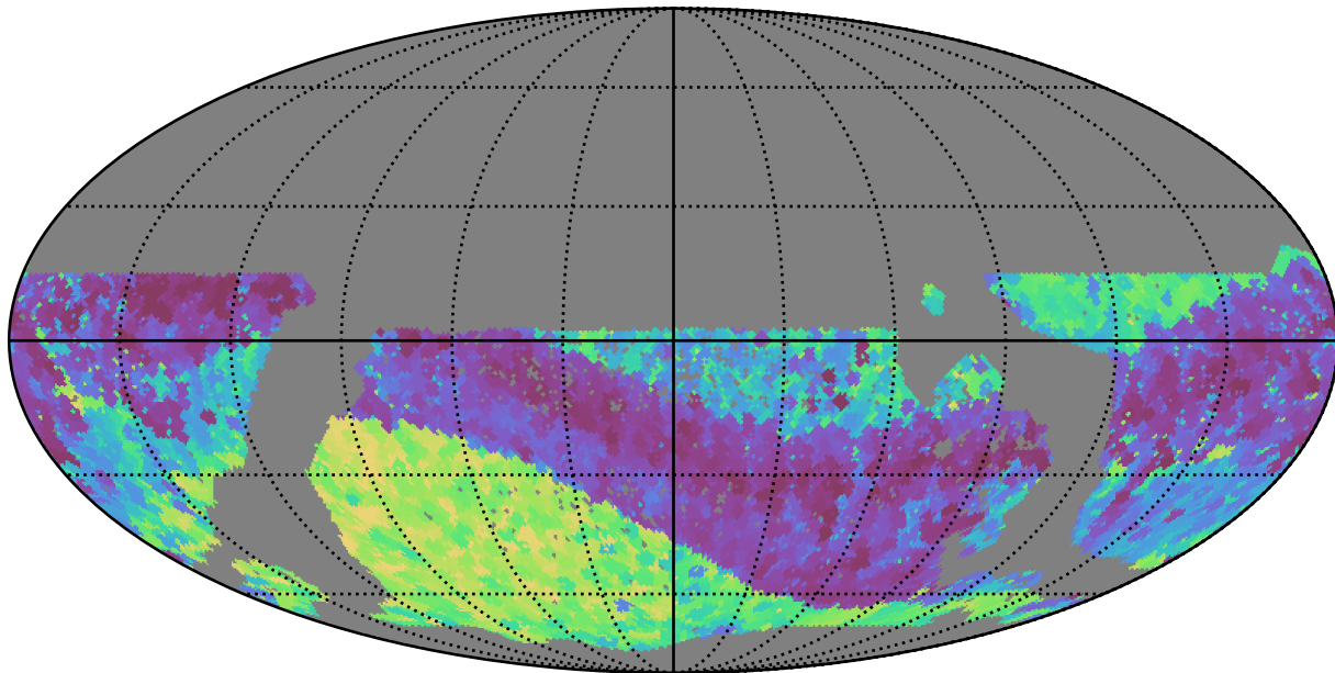
mw_roll_bulge_v3.3_10yrs WFD z band: Min skyBrightness
