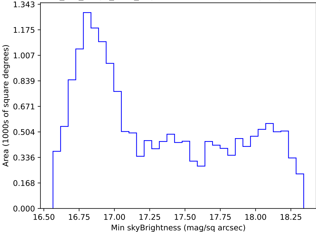
mw_roll_bulge_v3.3_10yrs WFD z band: Min skyBrightness
