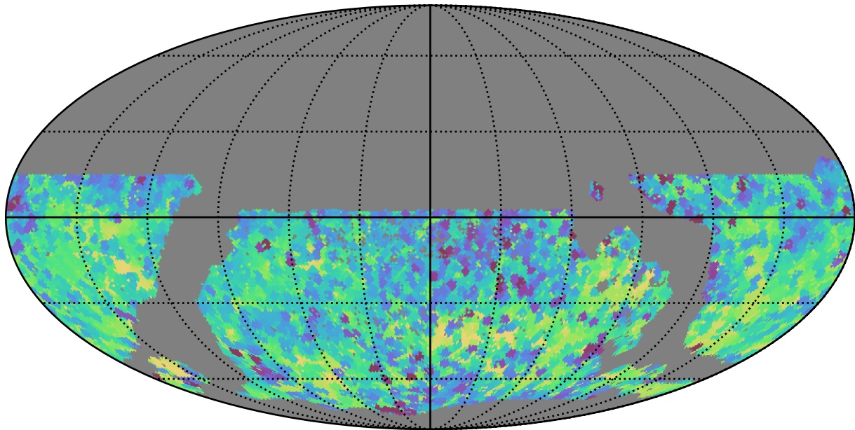
mw_roll_bulge_v3.3_10yrs WFD y band: Min skyBrightness
