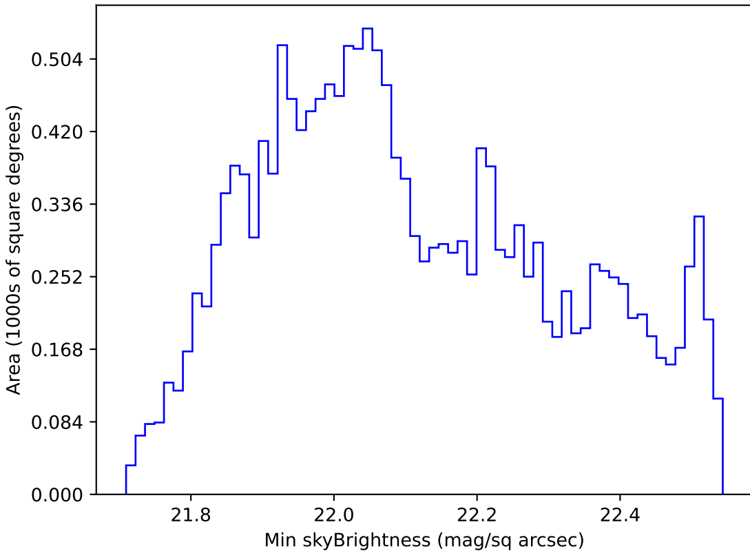
mw_roll_bulge_v3.3_10yrs WFD u band: Min skyBrightness
