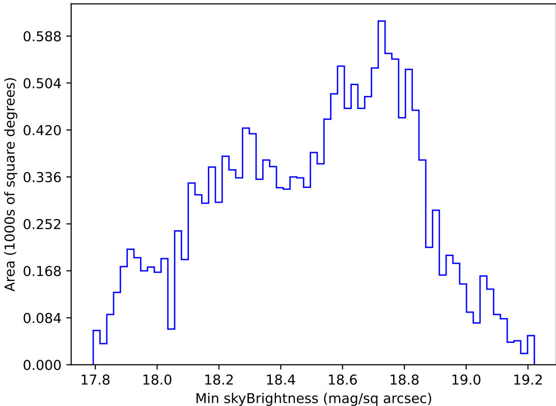
mw_roll_bulge_v3.3_10yrs WFD r band: Min skyBrightness
