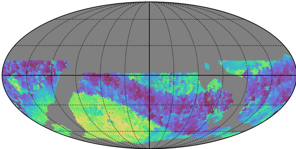
mw_roll_bulge_v3.3_10yrs WFD i band: Min skyBrightness
