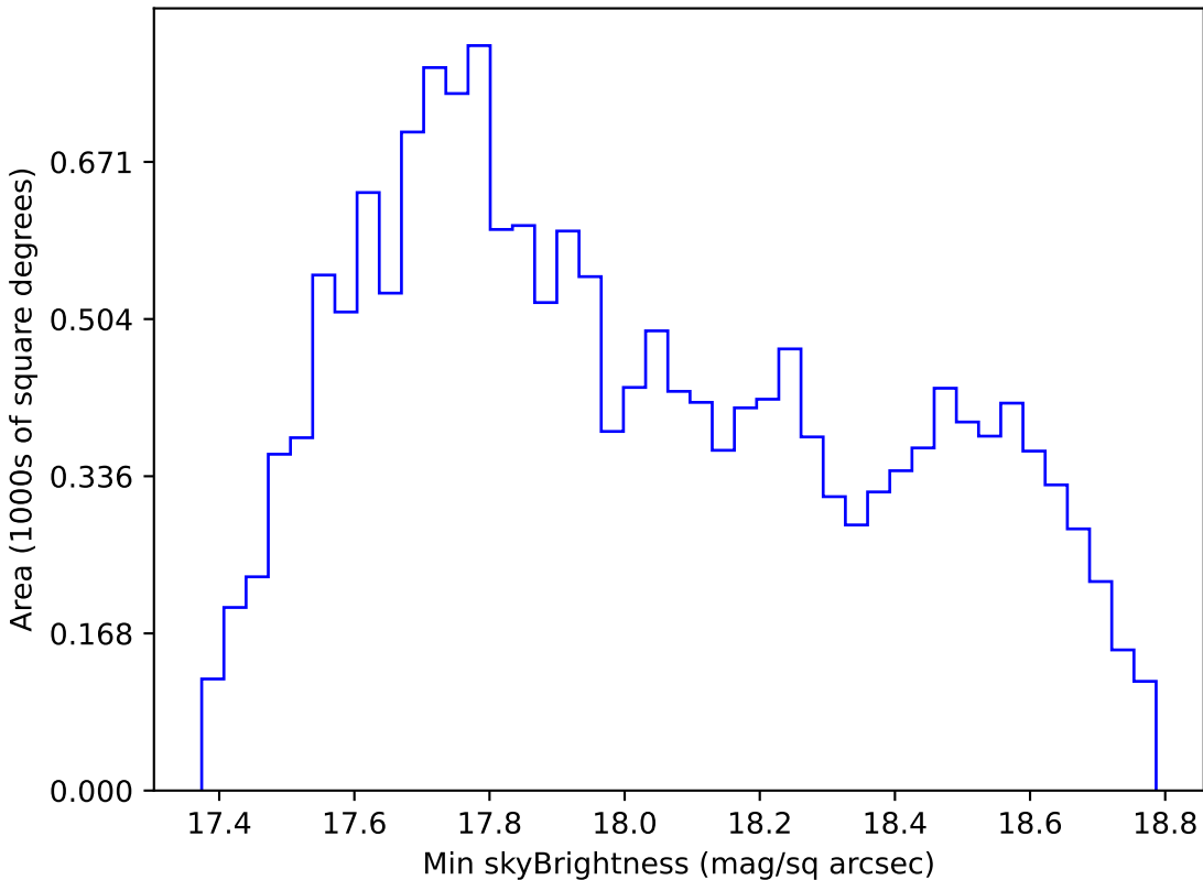
mw_roll_bulge_v3.3_10yrs WFD i band: Min skyBrightness
