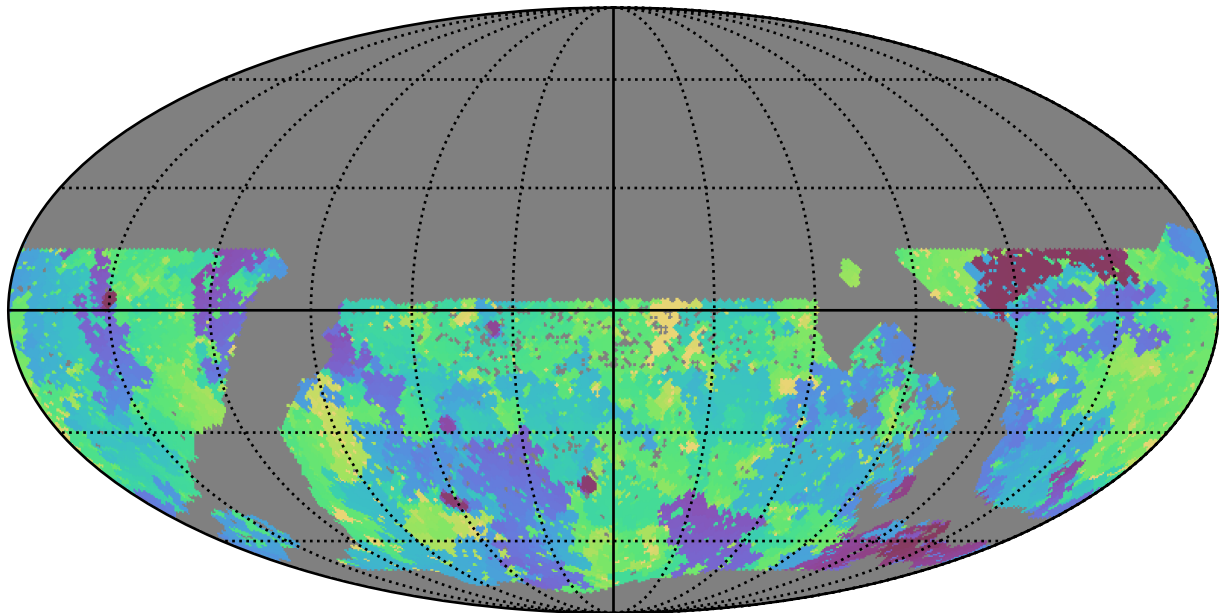
mw_roll_bulge_v3.3_10yrs WFD g band: Min skyBrightness
