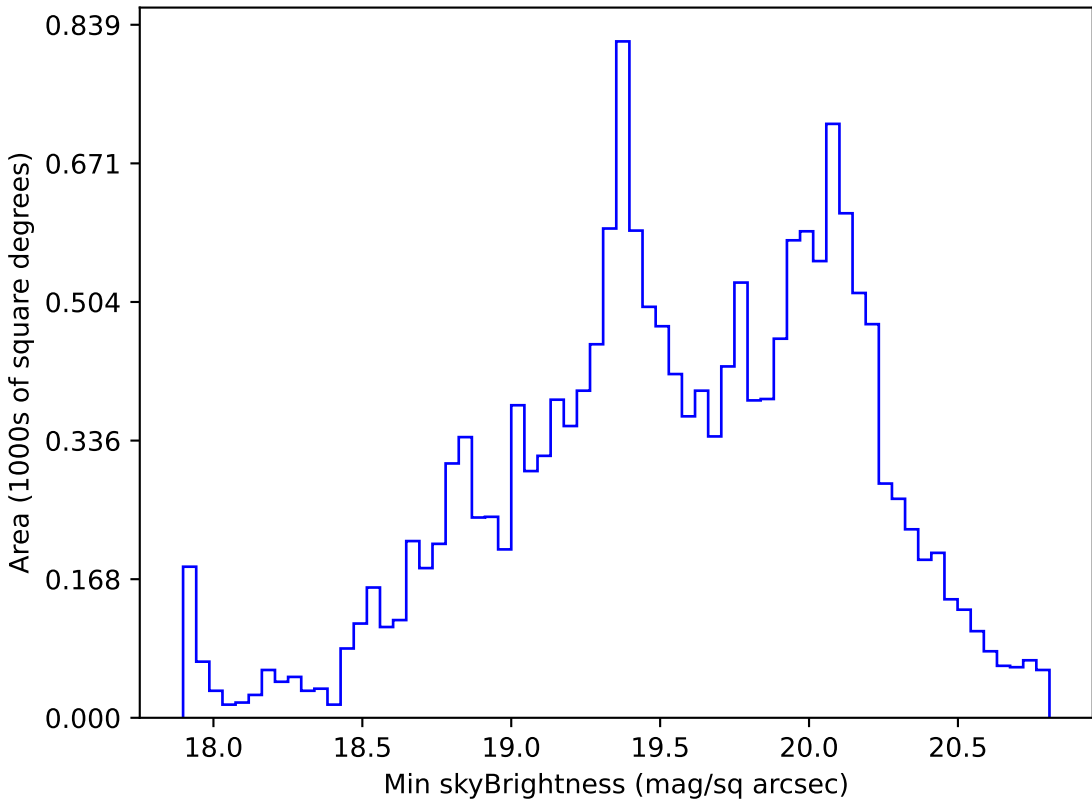
mw_roll_bulge_v3.3_10yrs WFD g band: Min skyBrightness
