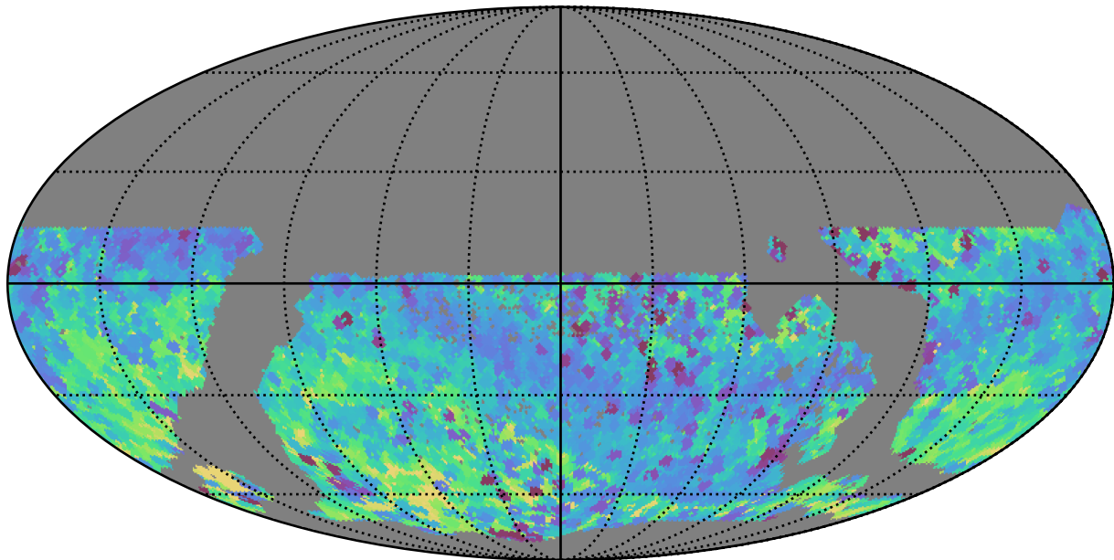
mw_roll_bulge_v3.3_10yrs WFD all bands: Min skyBrightness
