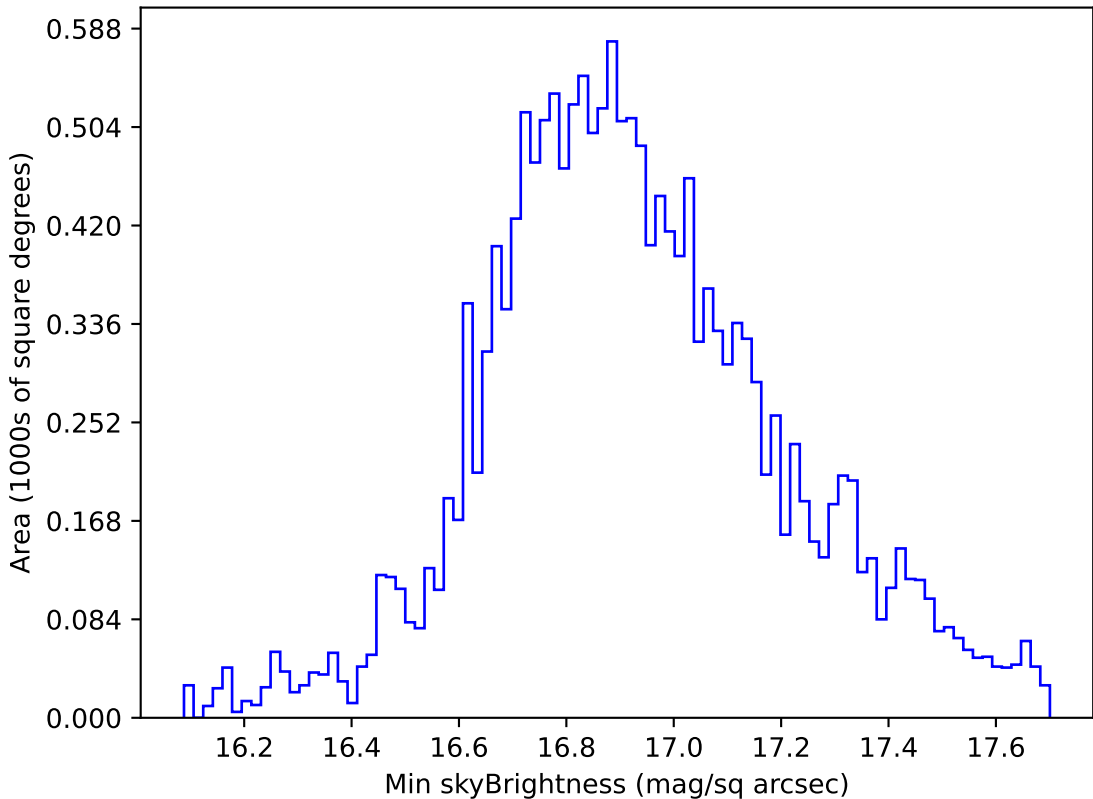
mw_roll_bulge_v3.3_10yrs WFD all bands: Min skyBrightness
