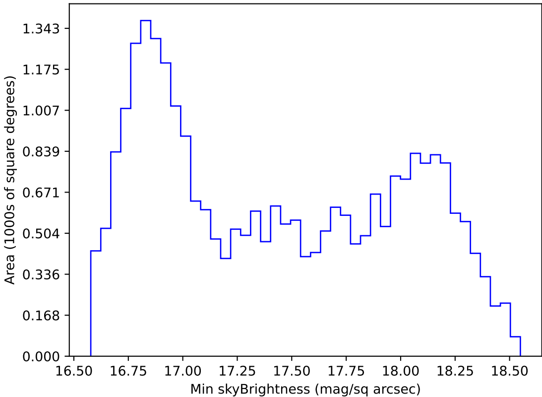
mw_roll_bulge_v3.3_10yrs All sky z band: Min skyBrightness
