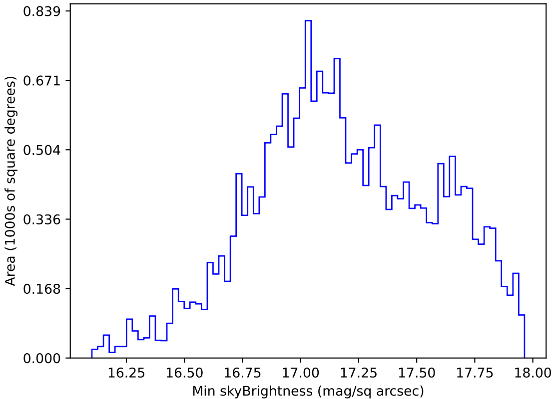
mw_roll_bulge_v3.3_10yrs All sky y band: Min skyBrightness
