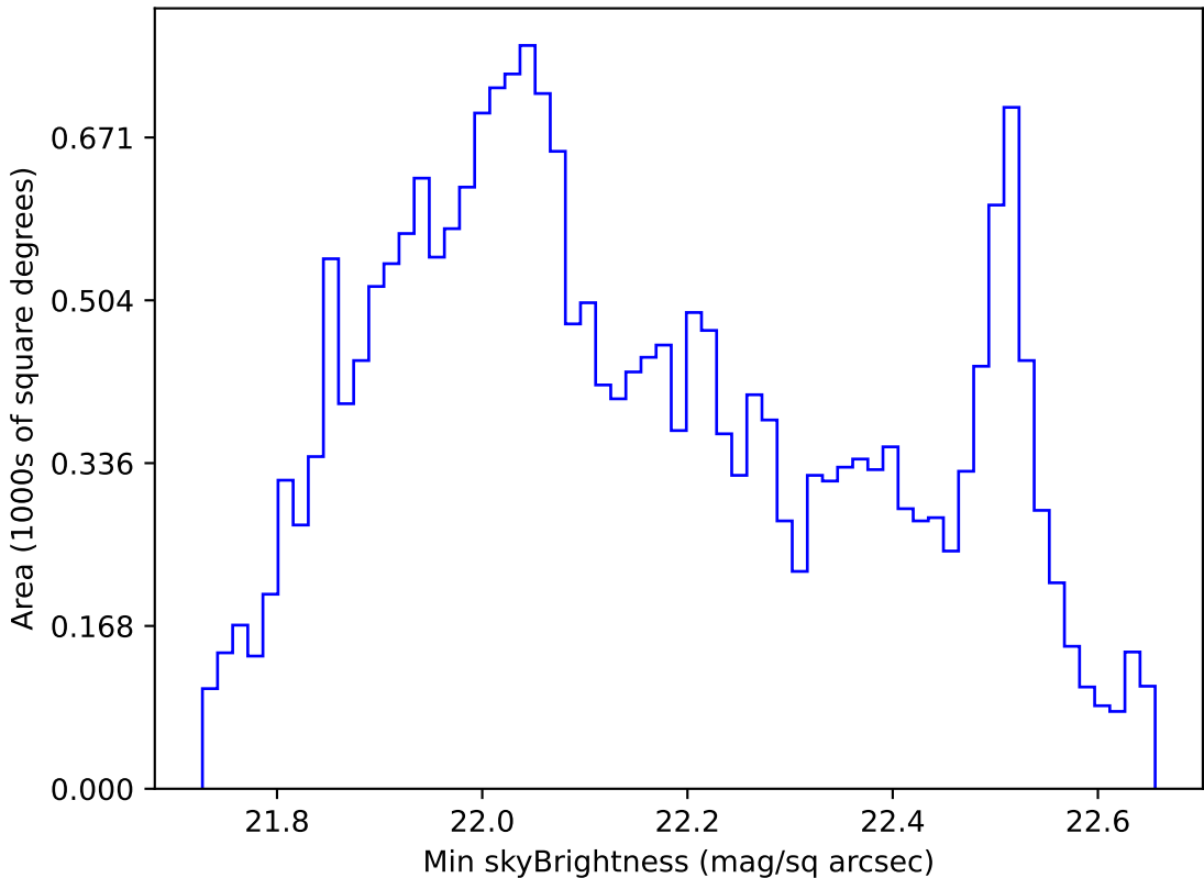
mw_roll_bulge_v3.3_10yrs All sky u band: Min skyBrightness
