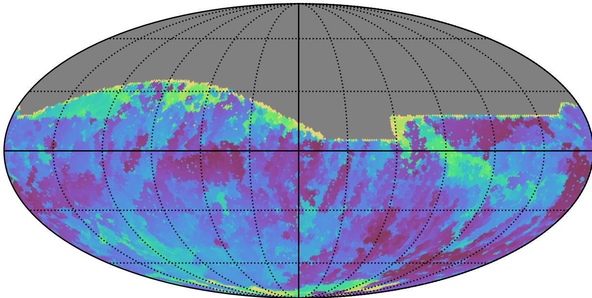
mw_roll_bulge_v3.3_10yrs All sky r band: Min skyBrightness
