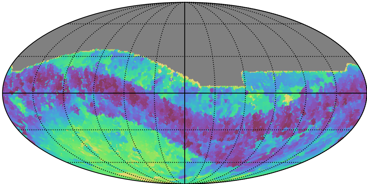
mw_roll_bulge_v3.3_10yrs All sky i band: Min skyBrightness
