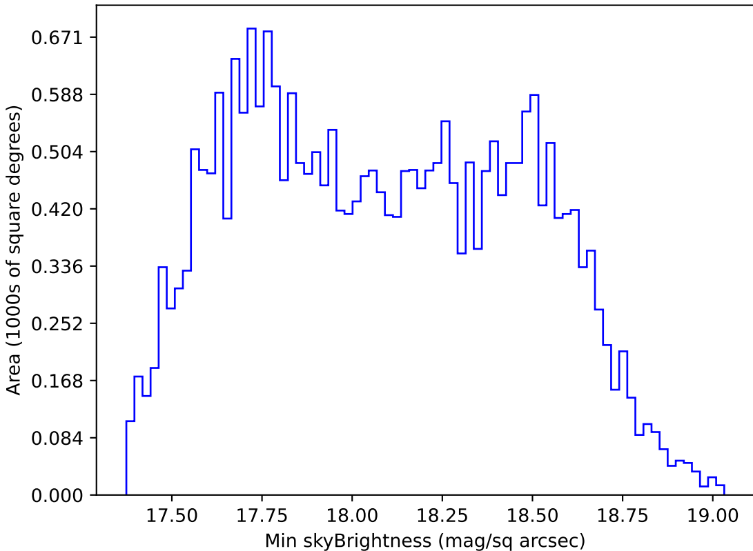
mw_roll_bulge_v3.3_10yrs All sky i band: Min skyBrightness
