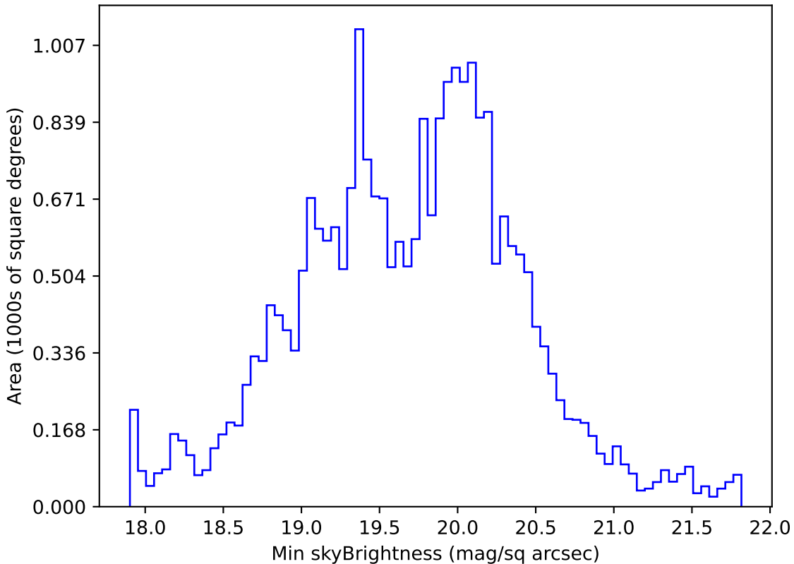
mw_roll_bulge_v3.3_10yrs All sky g band: Min skyBrightness
