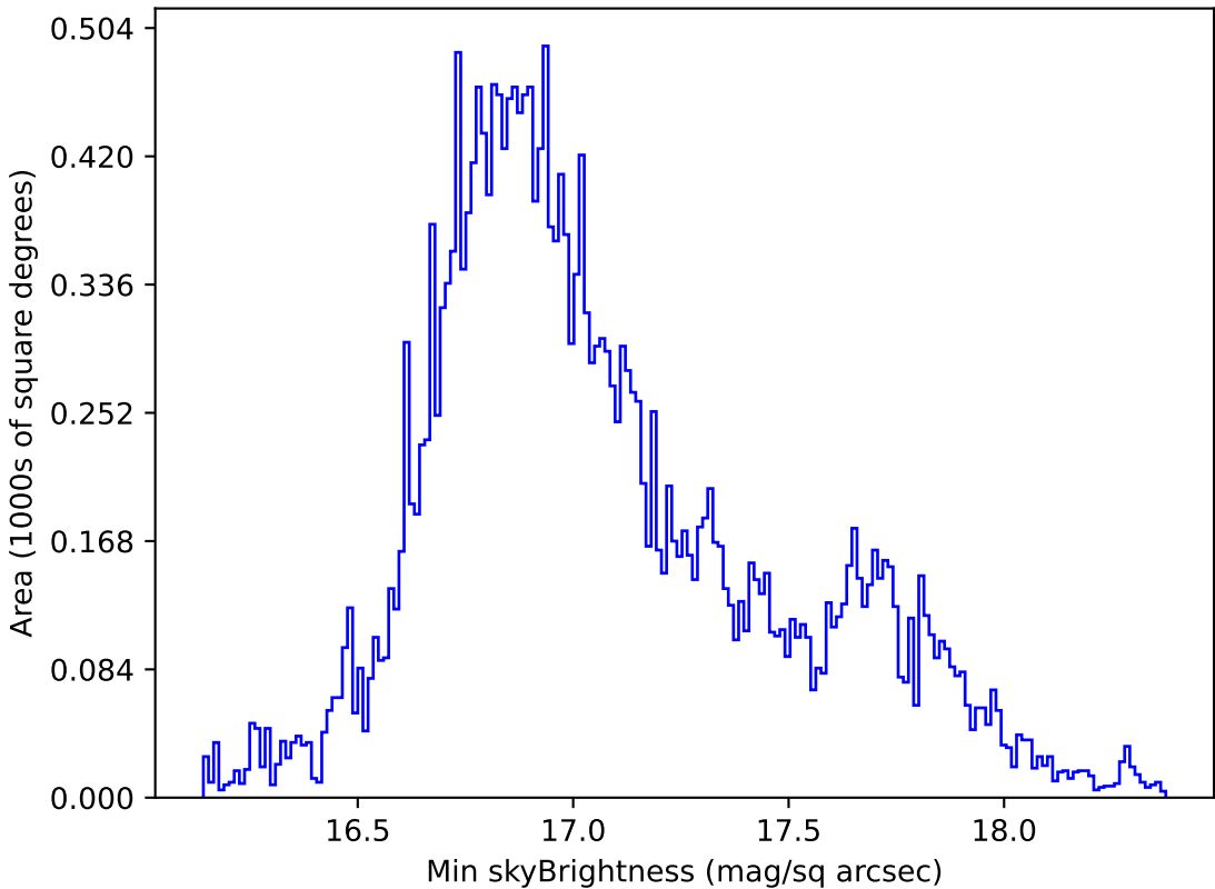
mw_roll_bulge_v3.3_10yrs All sky all bands: Min skyBrightness
