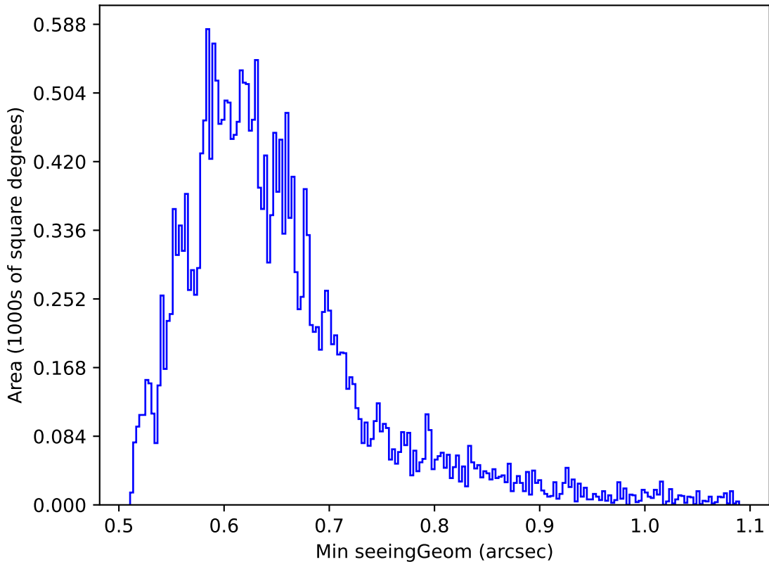
mw_roll_bulge_v3.3_10yrs Yr 1 z band: Min seeingGeom
