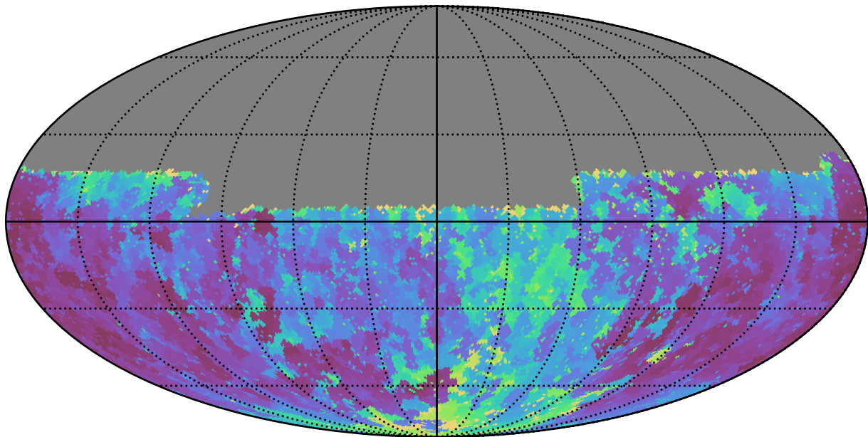
mw_roll_bulge_v3.3_10yrs Yr 1 u band: Min seeingGeom
