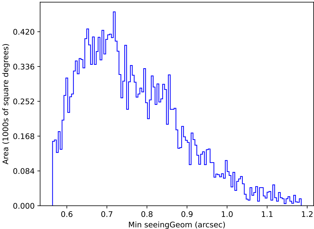
mw_roll_bulge_v3.3_10yrs Yr 1 u band: Min seeingGeom
