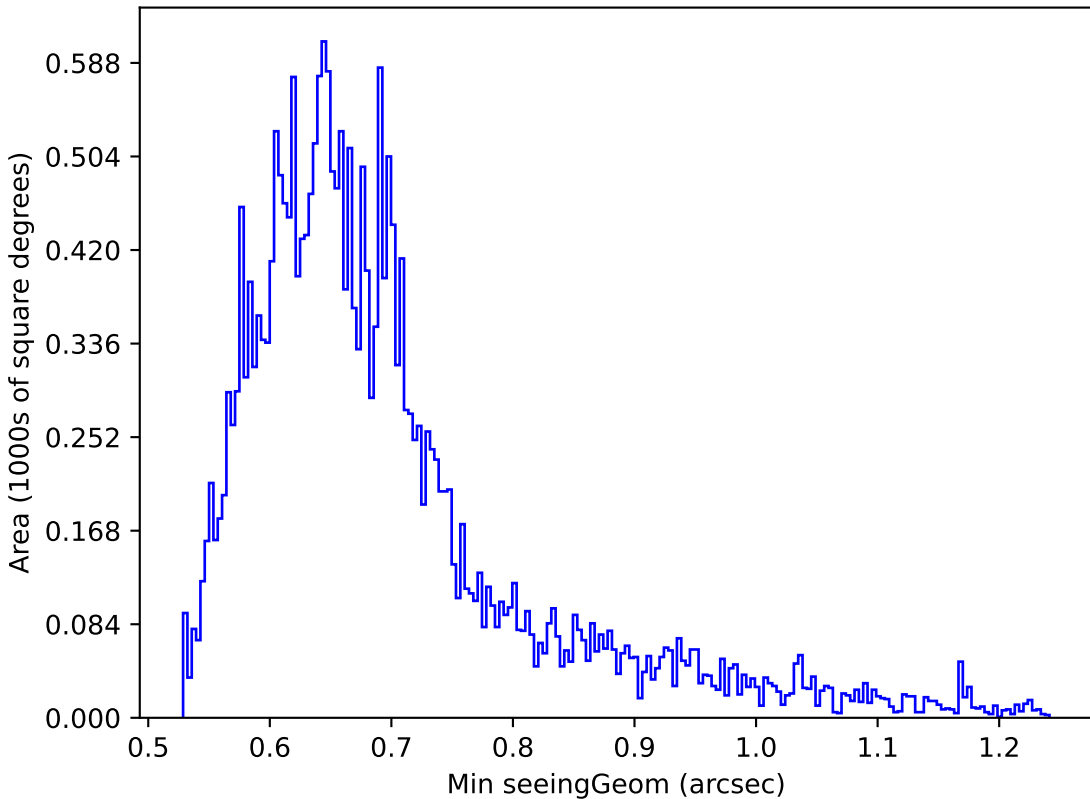
mw_roll_bulge_v3.3_10yrs Yr 1 g band: Min seeingGeom
