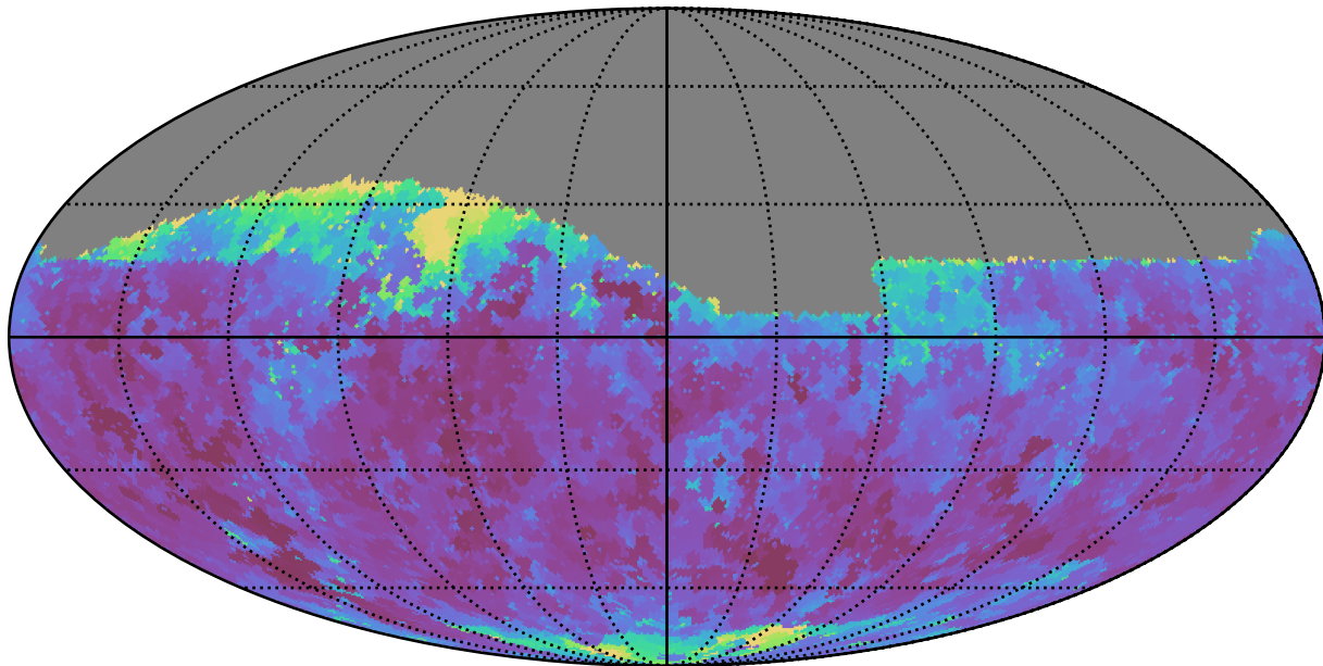
mw_roll_bulge_v3.3_10yrs Yr 1 z band: Min seeingEff
