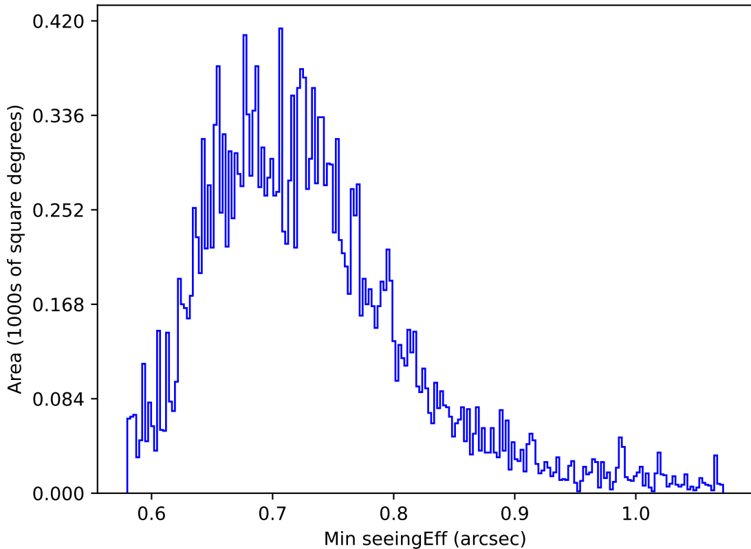
mw_roll_bulge_v3.3_10yrs Yr 1 y band: Min seeingEff
