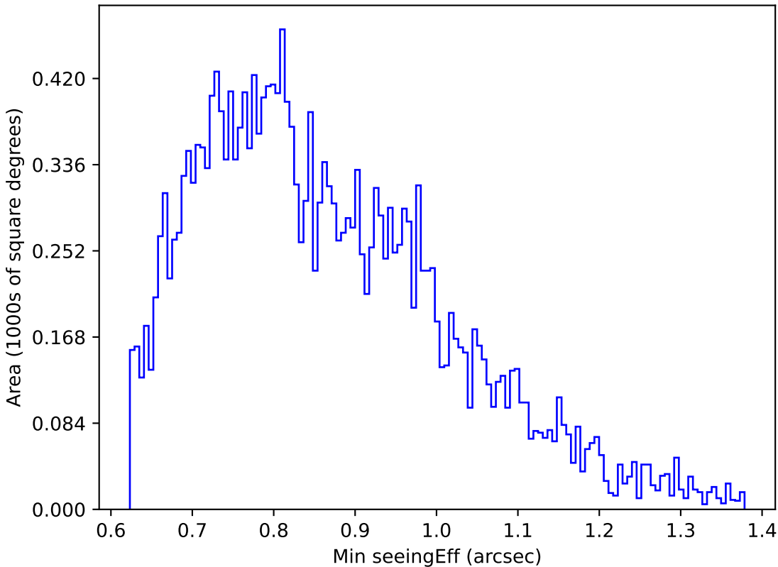
mw_roll_bulge_v3.3_10yrs Yr 1 u band: Min seeingEff
