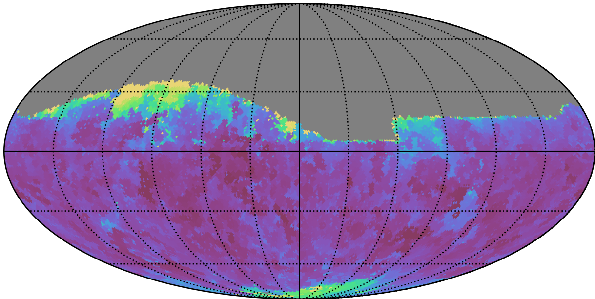
mw_roll_bulge_v3.3_10yrs Yr 1 r band: Min seeingEff
