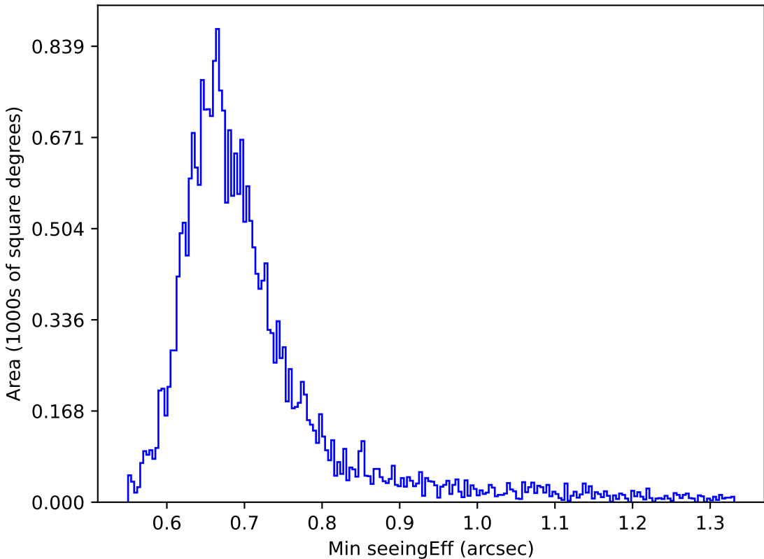
mw_roll_bulge_v3.3_10yrs Yr 1 r band: Min seeingEff
