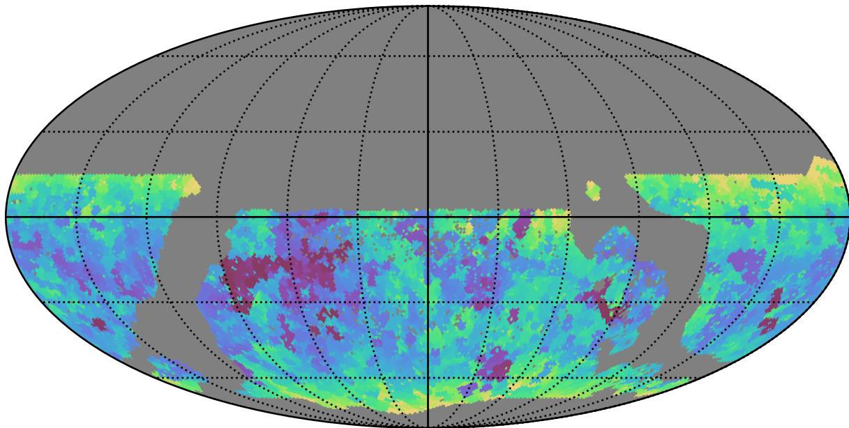
mw_roll_bulge_v3.3_10yrs WFD z band: Min seeingEff
