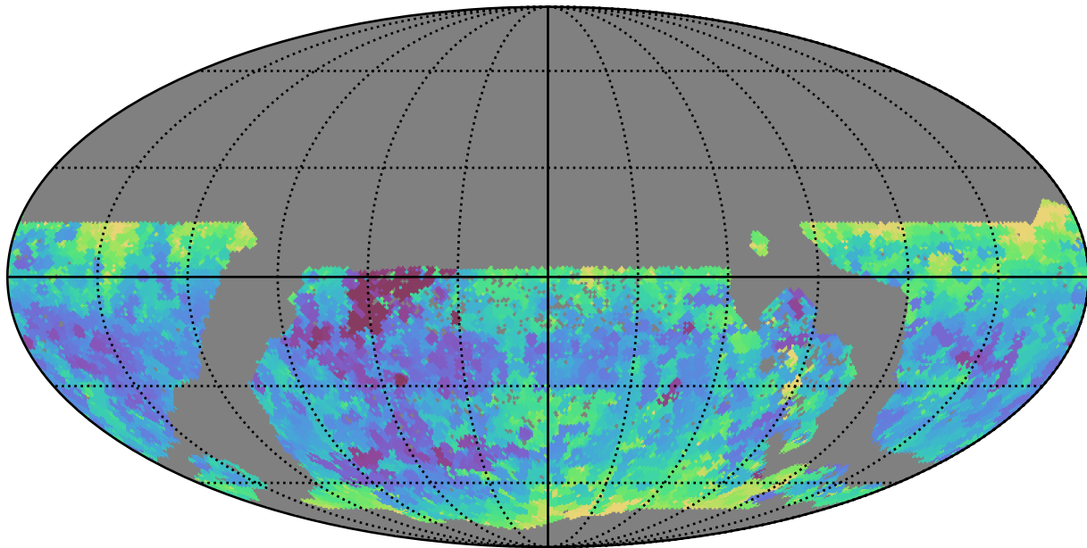
mw_roll_bulge_v3.3_10yrs WFD y band: Min seeingEff
