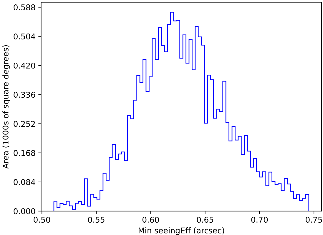
mw_roll_bulge_v3.3_10yrs WFD y band: Min seeingEff
