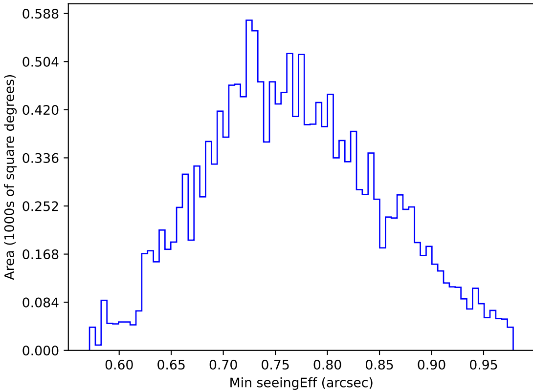
mw_roll_bulge_v3.3_10yrs WFD u band: Min seeingEff
