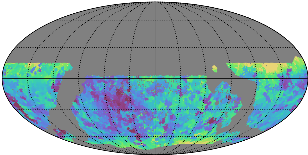
mw_roll_bulge_v3.3_10yrs WFD r band: Min seeingEff
