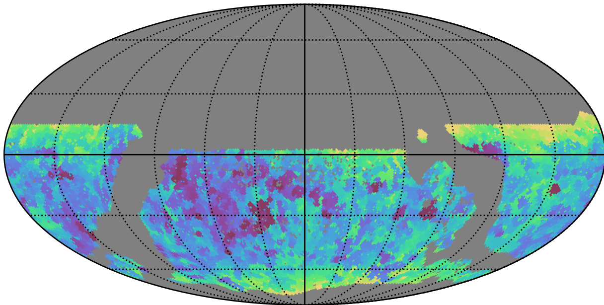
mw_roll_bulge_v3.3_10yrs WFD i band: Min seeingEff
