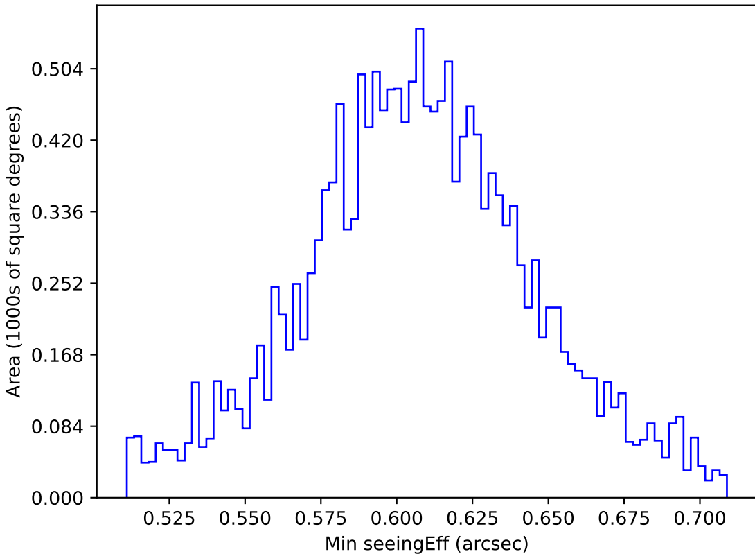
mw_roll_bulge_v3.3_10yrs WFD i band: Min seeingEff
