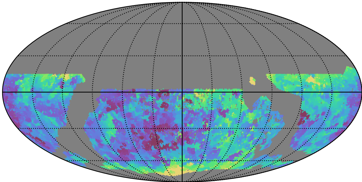
mw_roll_bulge_v3.3_10yrs WFD g band: Min seeingEff
